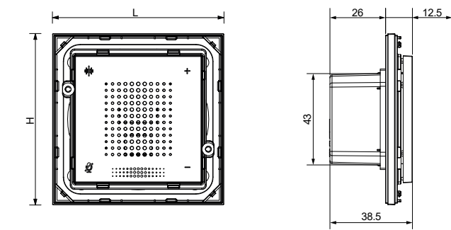
Mounting with frame: 81 x 77 (L x H) Mounting without frame (*NF): 80 x 80 (L x H)
